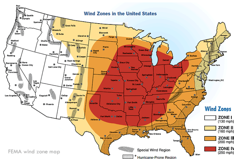
Figure 100: Wind Zones in the United States
